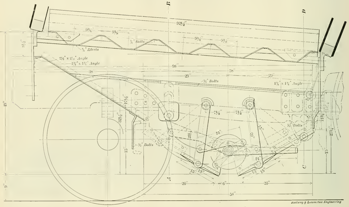
PLAYER ASH PAN
